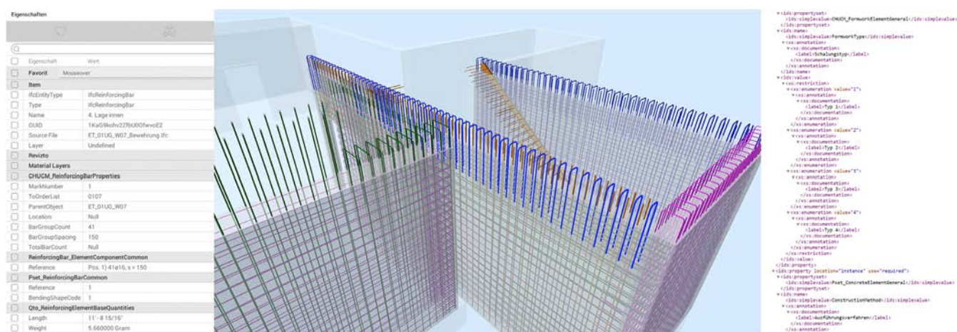
Fig. 3.65: Use Case »Model-based layout of reinforcement«
